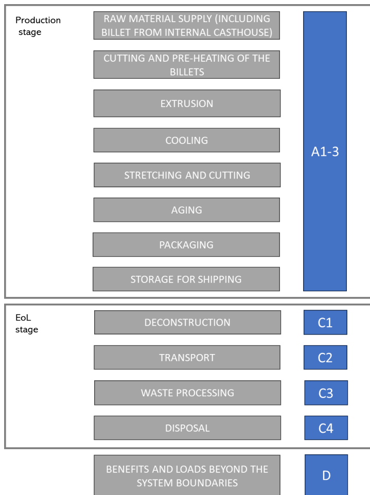
Figure 1. Scheme of the extrusion manufacturing process occurring at Cressona
