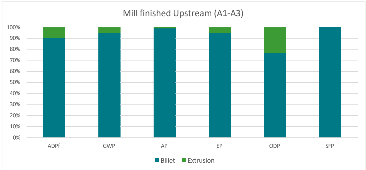
Figure 2. Relative contribution of upstream processes for mill-finished profile
