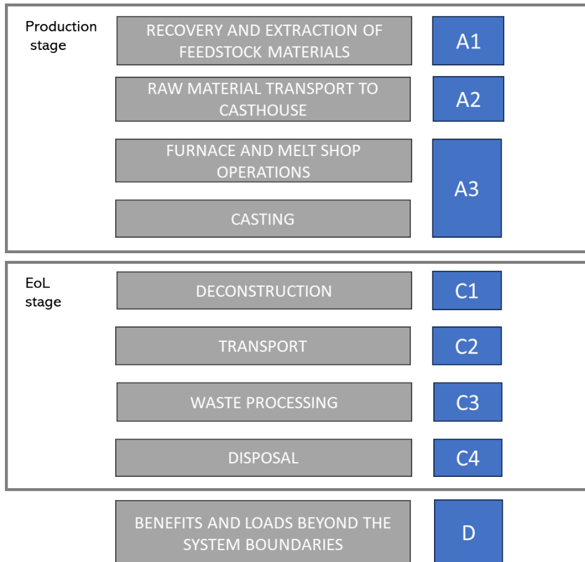
Figure 1. Scheme of the billet manufacturing process occurring at Phoenix Extrusion
